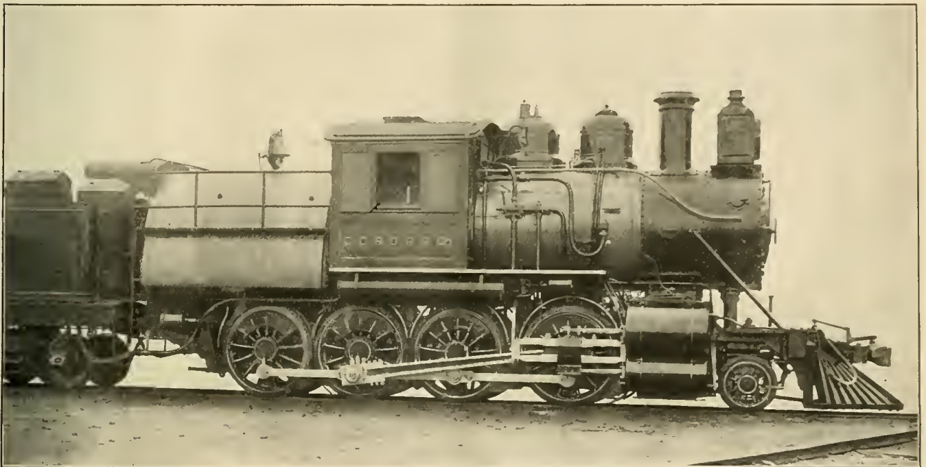
CHOCTAW, OKLAHOMA & GULF LOCOMOTIVE.
